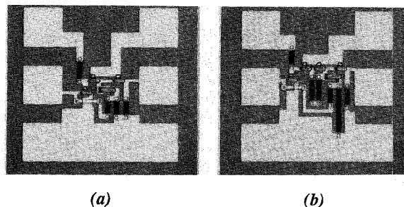
Fig. 2 Chip photographs of the basic-coupled buffer amplifier (a) and the Darlington-coupled buffer amplifier (b).
