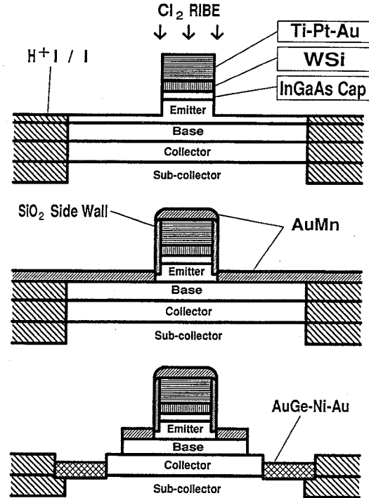
Fig. 3 Process flow for the self-aligned HBT fabrication.
